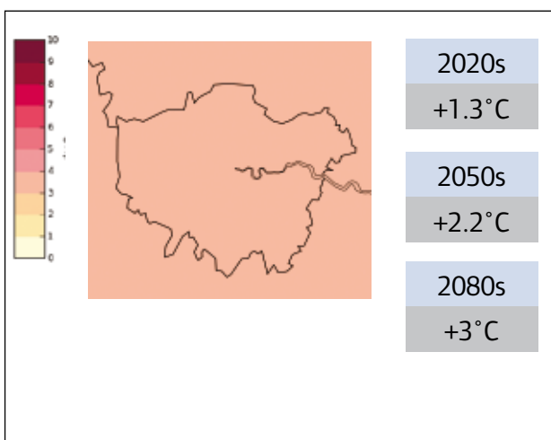
Figure 1.4 Changes in average winter temperature (°C) for London over the century compared to 1961-1990 baseline (central estimate, medium emissions scenario)
