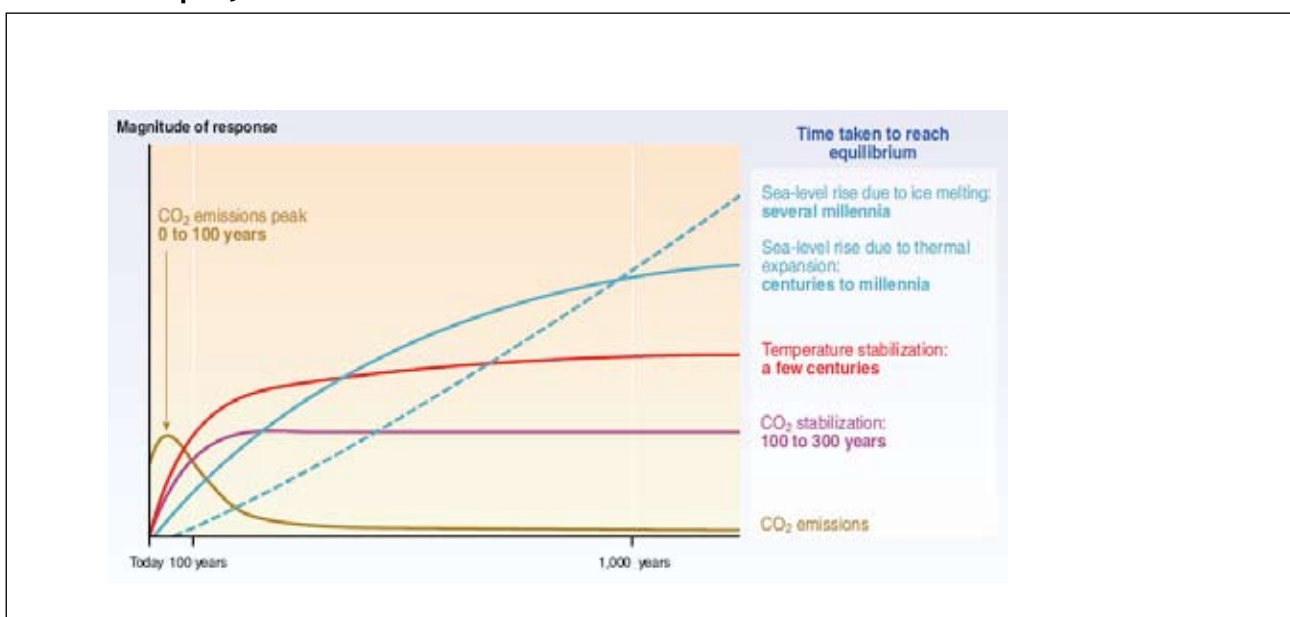
Figure 1.9. Climate system responses to reducing carbon dioxide (CO 2 ) emissions (source: IPCC Third Assessment Report)
