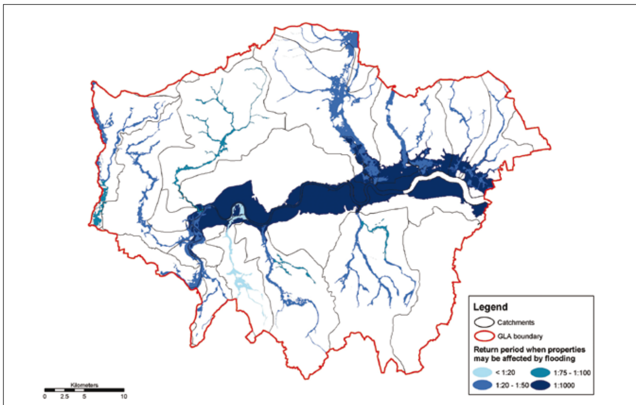
Figure 3.3 Area of London at risk of flooding, showing the different levels of probability, expressed as a return period (source: Environment Agency)
