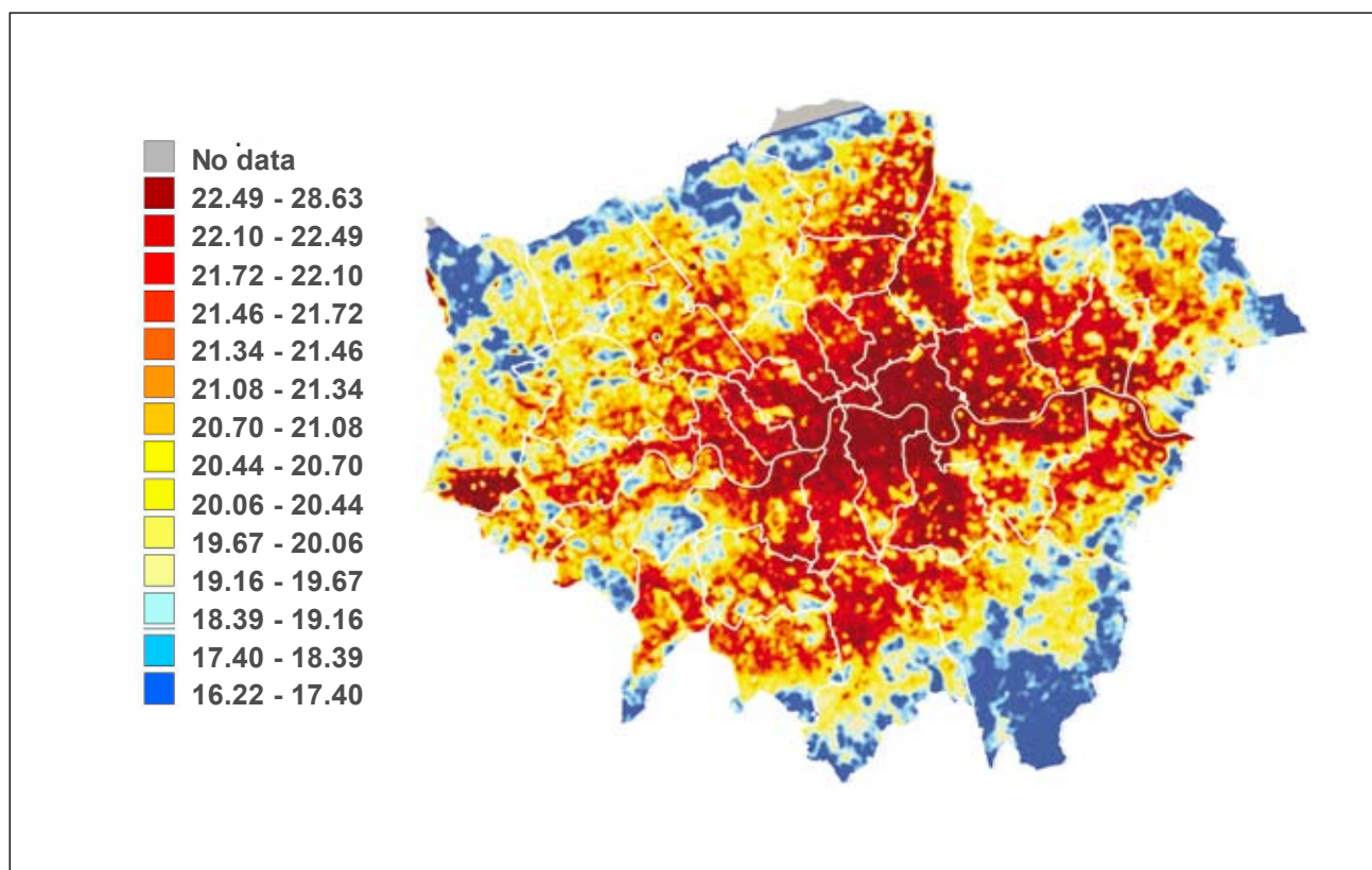
Figure 5.3 Surface temperature (°C) in London at 21.43pm on 12 July 2006 (source LUCID)
