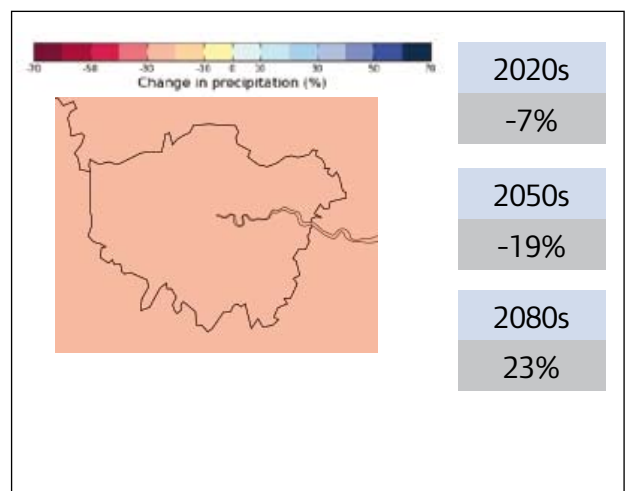
Figure 1.6 Changes to winter rainfall (percentage change against baseline) for London over the century compared to 1961-1990 baseline (central estimate, medium emissions scenario)
