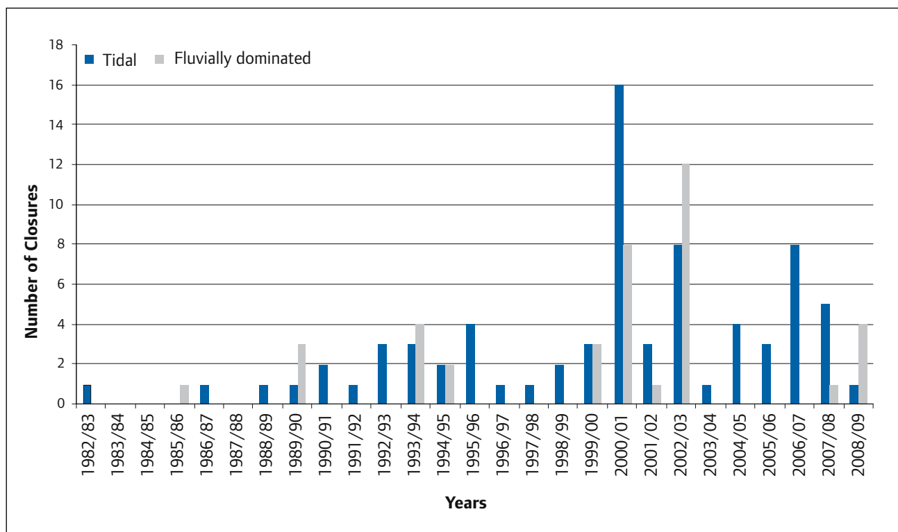
Figure 3.2 Thames Barrier closures 1982/83 to 2008/09 (source: Environment Agency)
