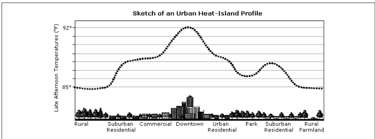
Figure 5.2 Typical temperature profile of an urban heat island
