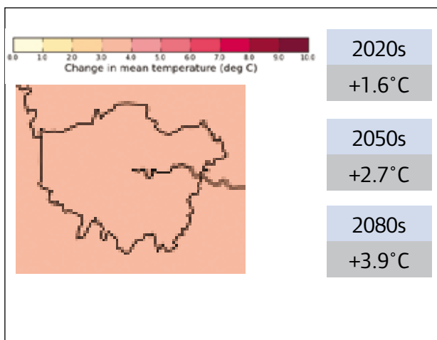
Figure 1.3. Changes in average summer temperature (°C) for London over the century compared to 1961-1990 baseline (central estimate, medium emissions scenario)
