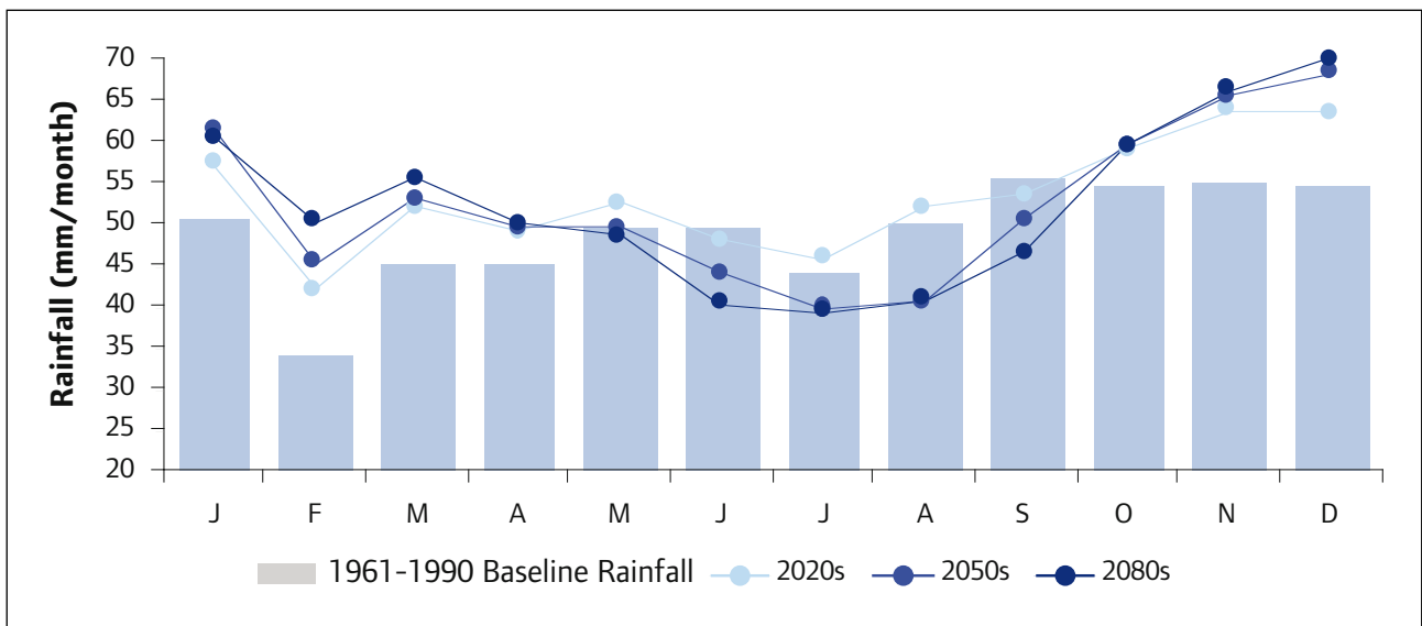
Figure 1.8 Average monthly rainfall (mm of rainfall per month) in London over the century, under a medium emissions scenario, compared to baseline period.
