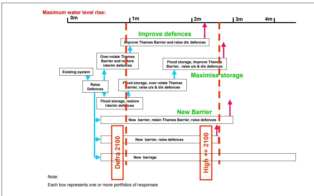
Figure 3.6 TE2100 'decisions pathway'. The flood risk management options are plotted against the maximum level of protection against sea level rise that they can provide. The right hand dotted line shows the worst case sea level rise scenario to the end of the century (u/s = upstream, d/s = downstream) (source: Environment Agency).
