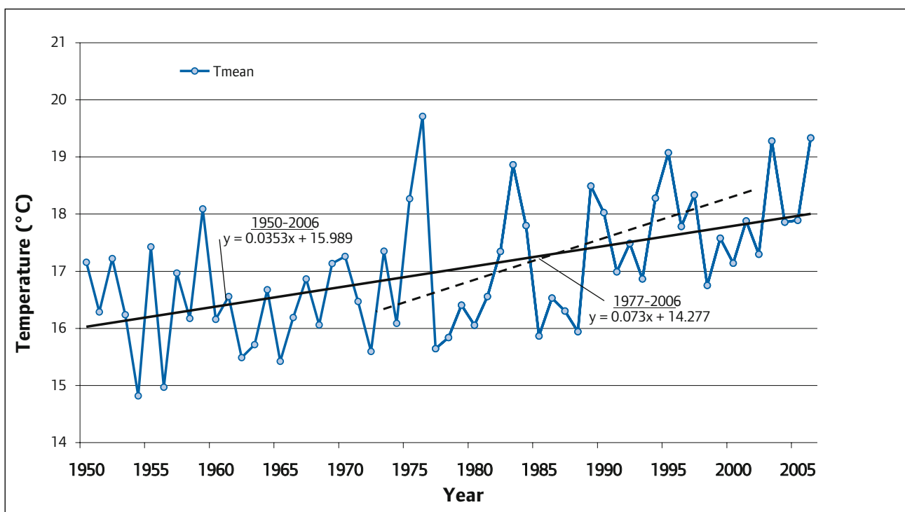
Figure 1.2 Average summer temperatures in London 1950–2006 (source: Met Office)
